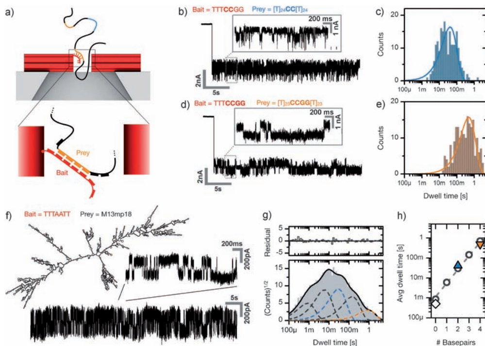
Figure 3. Sequence-specific prey DNA detection with functionalized DNA nanopores on SiN nanopores.
