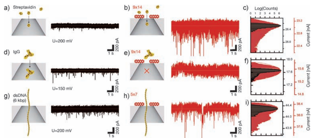
Figure 2. DNA nanoplates with custom apertures for size-selective macromolecular sensing with SiN nanopores. a) Current–time traces observed for streptavidin ( cis concentration = 20 nM) translocation through bare nanopores, b) Current–time traces after insertion of a nanoplate with a central aperture of width 9 nm and length 14 nm (see Figure S5 for design details). c) Histogram of observed current levels. d–f) As in (a)–(c), but with Immunoglobulin G (IgG; cis concentration = 20 nM). g–i) As in (a)–(c), but with 6 kbp linear double-helical DNA molecules ( cis concentration = 300 pM) and a nanoplate with aperture width 5 nm and length 7 nm (Figure S2, version 0).
